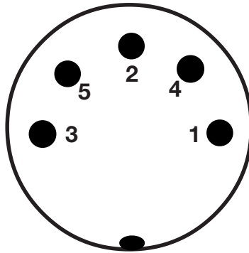
MALE PLUG FRONT VIEW
