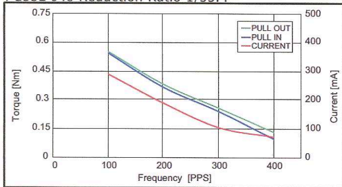
PG35L-048 Reduction Ratio 1/35.4
