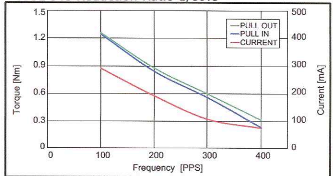
PG35L-048 Reduction Ratio 1/89.8
