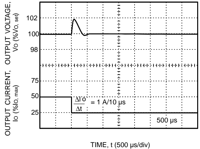
Figure 16. JC030A, B, C-M Typical Output Voltage for a Step Load Change from 50% to 25%
