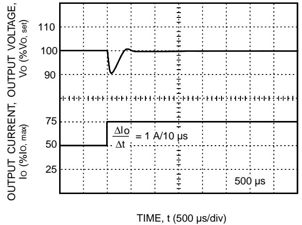
Figure 15. JC030D-M Typical Output Voltage for a Step Load Change from 50% to 75%
