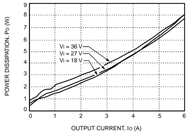
Figure 28. JC030A-M Power Dissipation vs. Output Current
