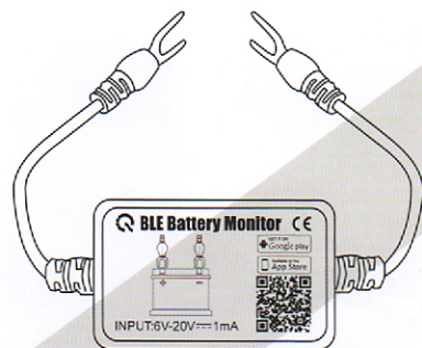
Battery Monitor
