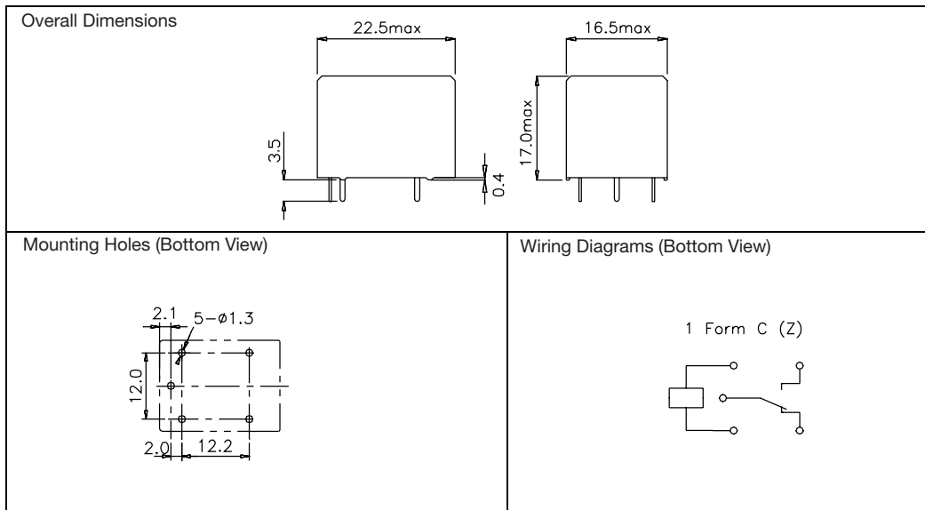
OVERALL DIMENSIONS, MOUNTING HOLES AND WIRING DIAGRAMS (mm)
