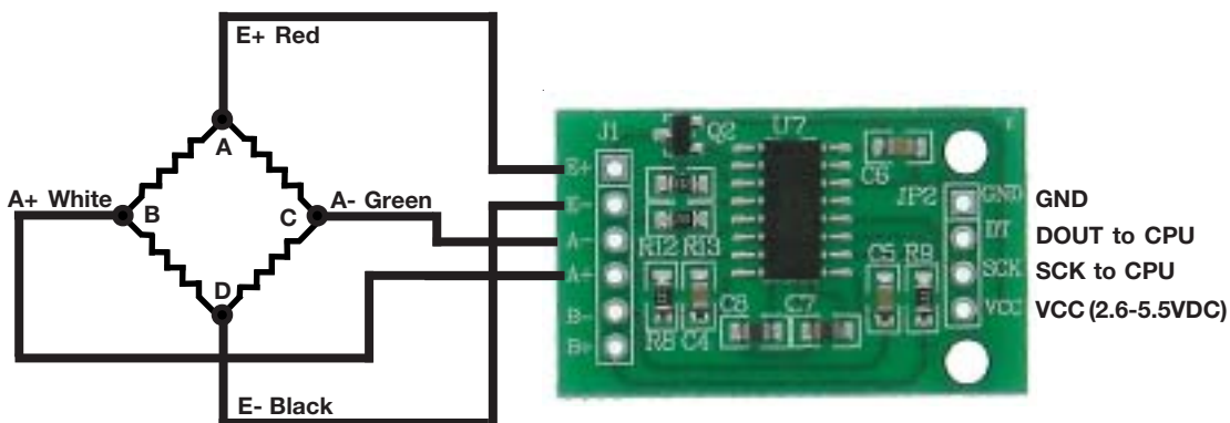
Figure 4: Connections
