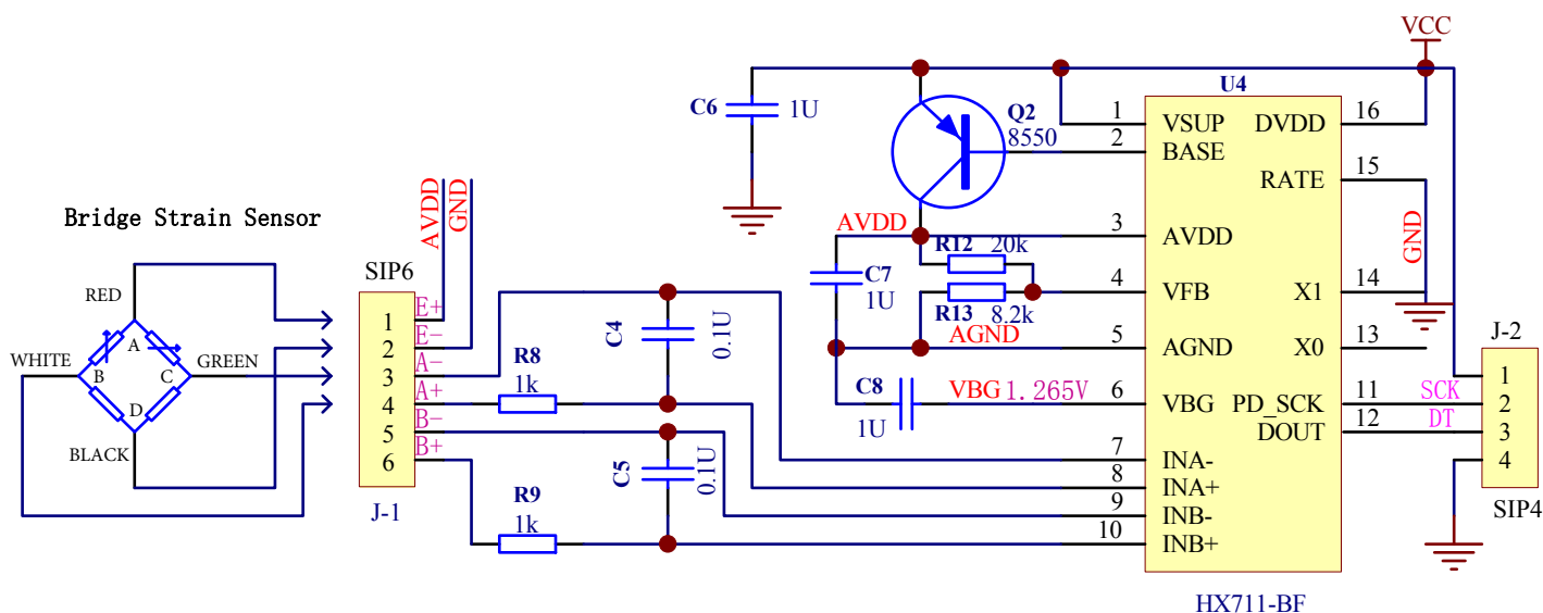
Figure 5: Schematic
