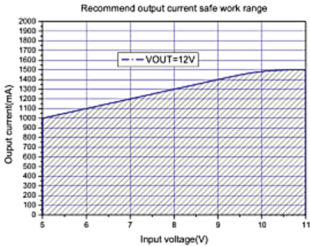
Max output Current (VOUT=12V)
