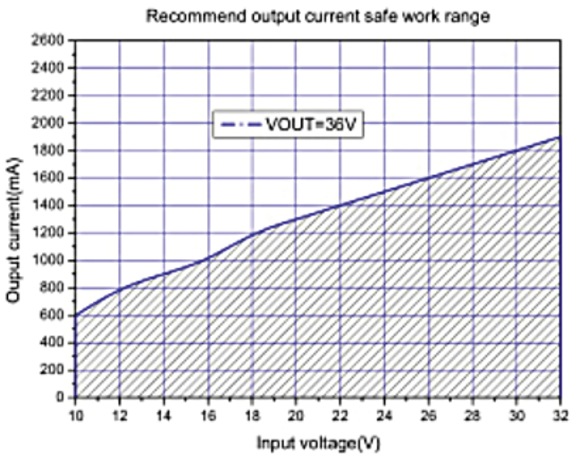
Max output Current (VOUT=36V)
