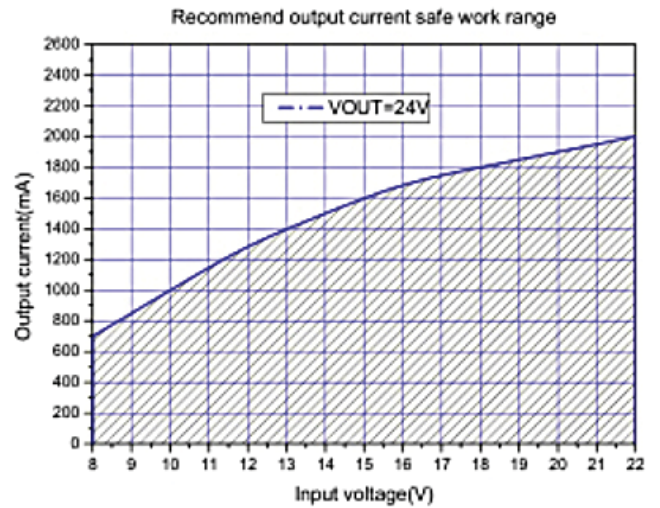
Max output Current (VOUT=24V)
