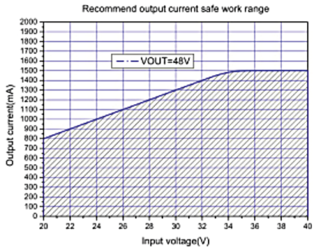
Max output Current (VOUT=48V)
