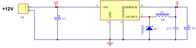
ONBOARD +5V POWER SUPPLY
