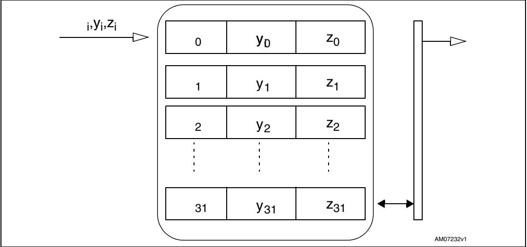
Figure 8. FIFO mode
