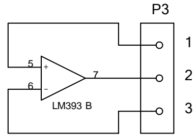
EXTRA COMPARATOR
