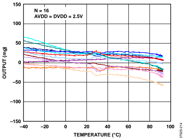
Figure 14. Y-Axis Zero g Offset vs. Temperature— Eight Parts Soldered to PCB, V_S = 2.5\text{ V}
