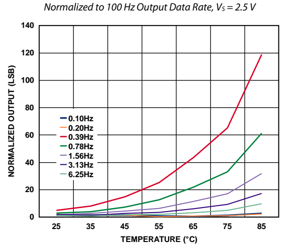
Figure 54. Typical Y-Axis Output vs. Temperature at Lower Data Rates, Normalized to 100 Hz Output Data Rate, V_s = 2.5\text{ V}
