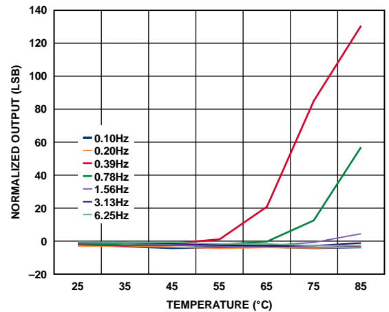
Figure 55. Typical Z-Axis Output vs. Temperature at Lower Data Rates, Normalized to 100 Hz Output Data Rate, V_s = 2.5\text{ V}
