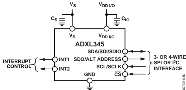
Figure 43. Application Diagram
