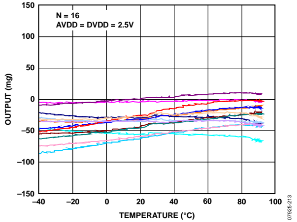
Figure 13. X-Axis Zero g Offset vs. Temperature— Eight Parts Soldered to PCB, V_S = 2.5\text{ V}
