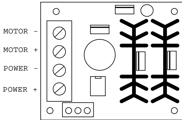
SPEED ADJ. 100K POT
