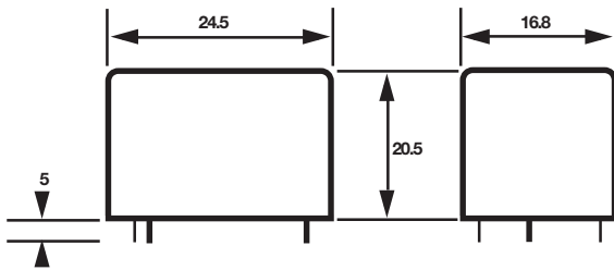
GENERAL DIMENSIONS
