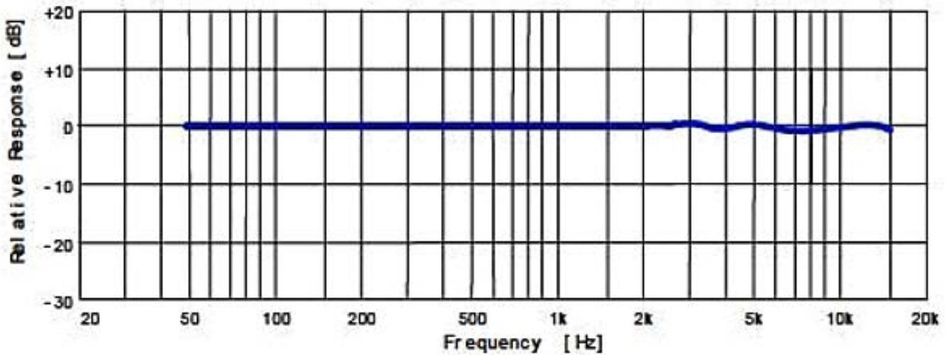
Mic Capsule
