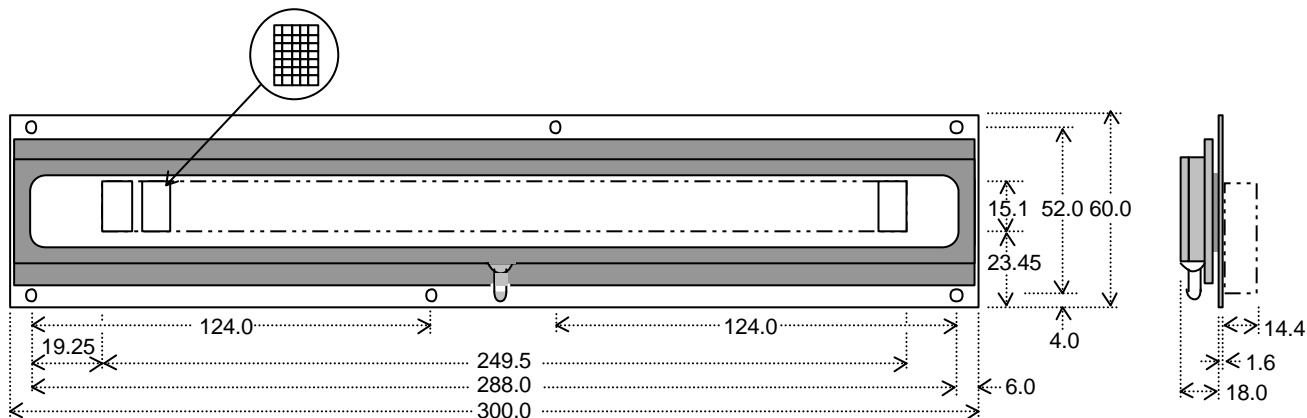
Dimensions in mm & subject to tolerances. Mounting holes 3.5mm dia.
